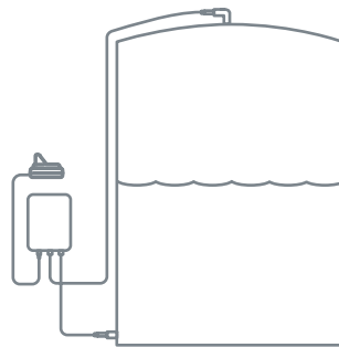
External Mount Bottom Sensor
